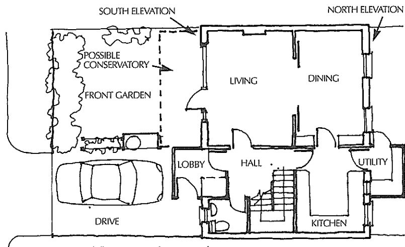
Ground floor - South aspect house
